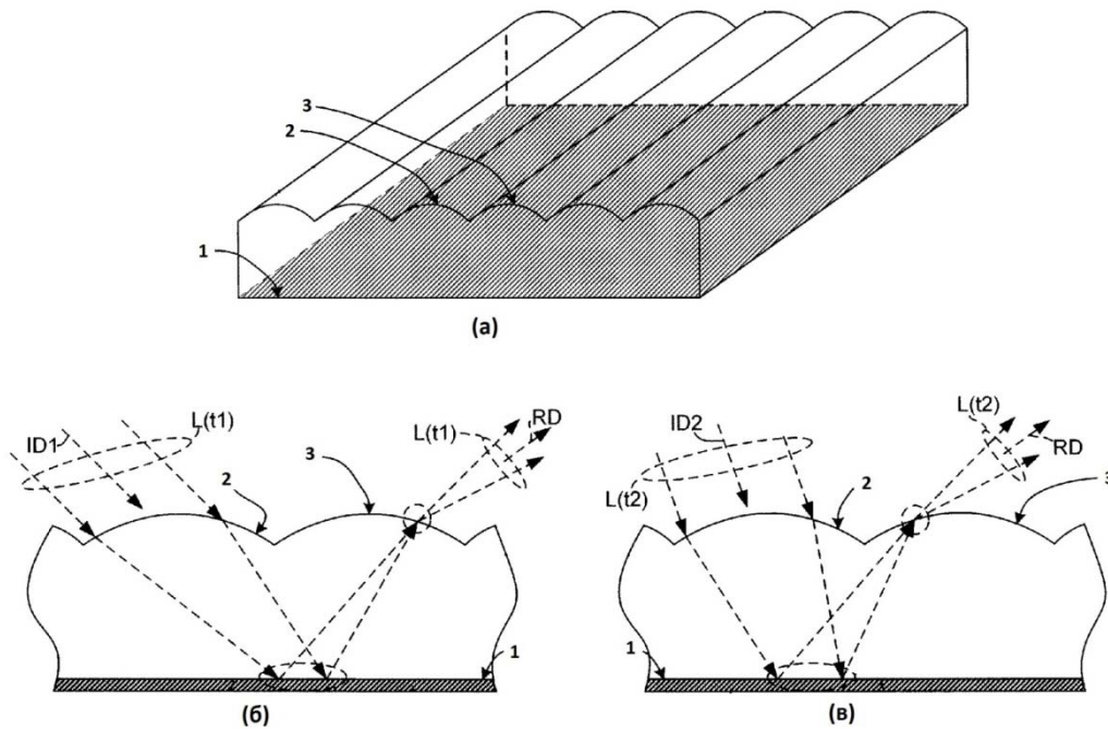
Figure 3 – Design model of the redirecting surface:
