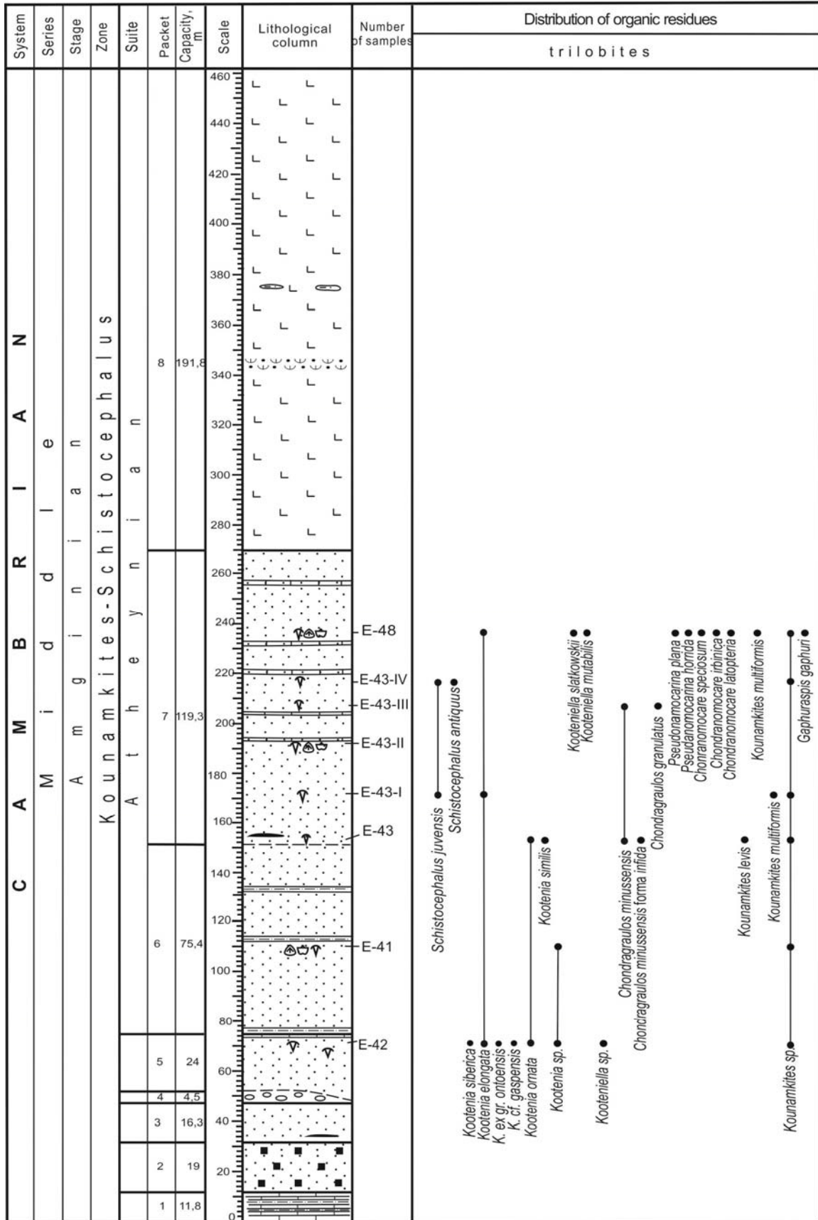
Figure 4 – Lithostratigraphic column with vertical range of the trilobite in the Athey suite of the Middle Cambrian (legend to column is described in figure 3)
