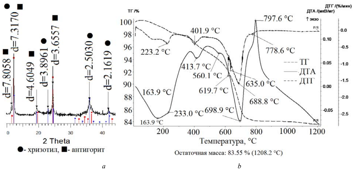
Figure 2 – Diffractogram - a and derivatogram - b of the averaged overburden rocks
