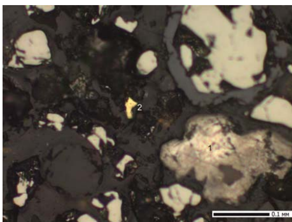
Figure 5 – Light yellow AgI (1), overgrown with porous AgII. 2 – yellow - high-grade gold. Uv. 200. Analysts Levin V.L., Kotelnikov P.E.
