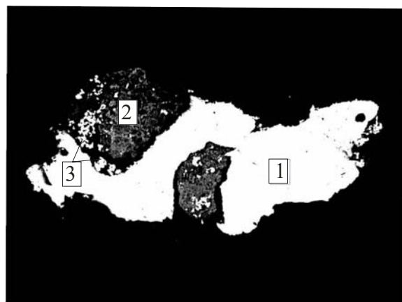
Figure 6 – Electrum swarm (1) and native silver (2) with fine inclusions of high-grade gold (3). Uv. 500. Analysts Levin V.L., Kotelnikov P.E.
