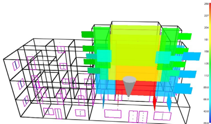
Figure 4 – Time layout of dangerous fire factors in the auditorium of the Lviv State Palace of Aesthetic Education of Youth
